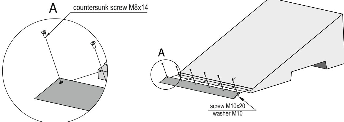
Rys. 1 Steel toe plate assembly scheme.
