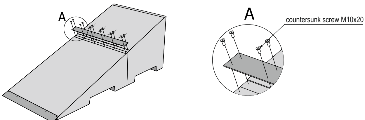
Fig. 3 The additional element and Bank 600 connecting scheme.
